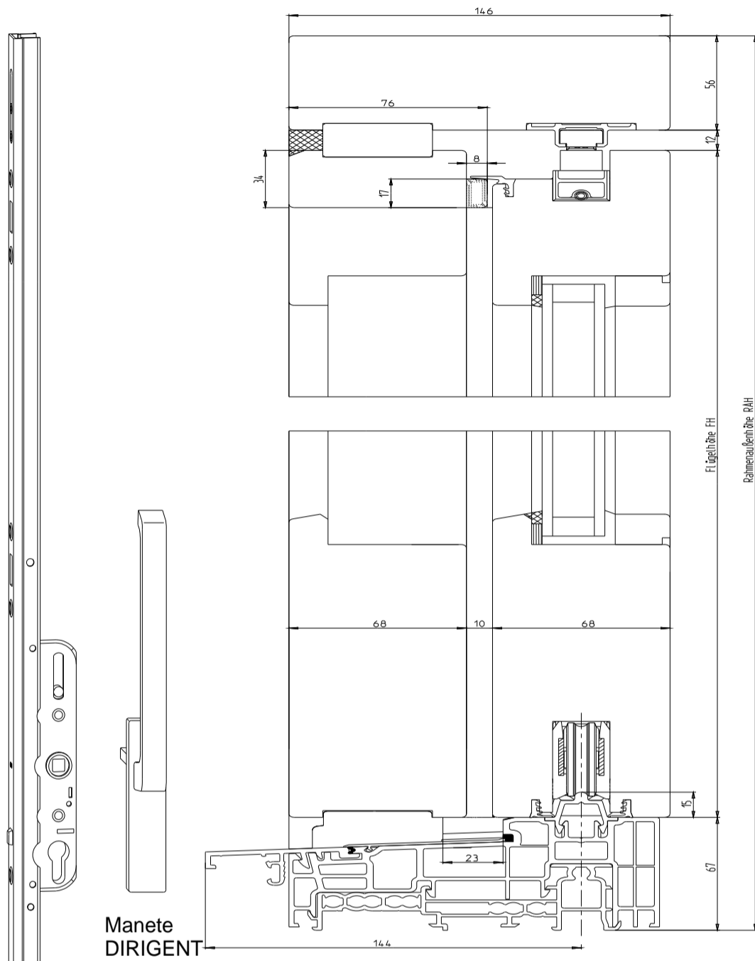
Corte Vertical
